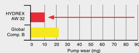
HYDREX AW Wear Protection vs. Competing Oils Eaton 35VQ25 Hydraulic Pump Wear Test
