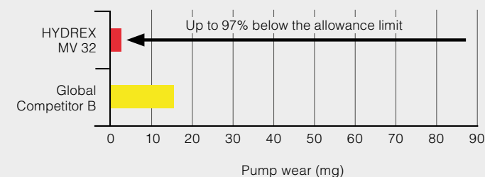
Eaton 35VQ25 Hydraulic Pump Wear Test
