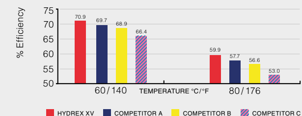
Overall Pump Efficiency of Multigrade Fluids (Parker Denison T6CM B06 vane pump, 1500 rpm, 250 bars / 3625 psi)
