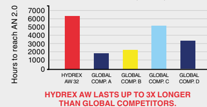
HYDREX AW Oxidation Life vs. Competing Oils ASTM D943 Test (ISO 32)
